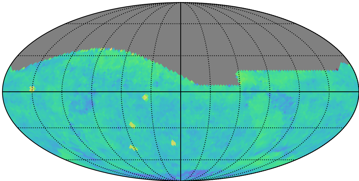
baseline_v3.0_10yrs (g or r or i): PairFraction
