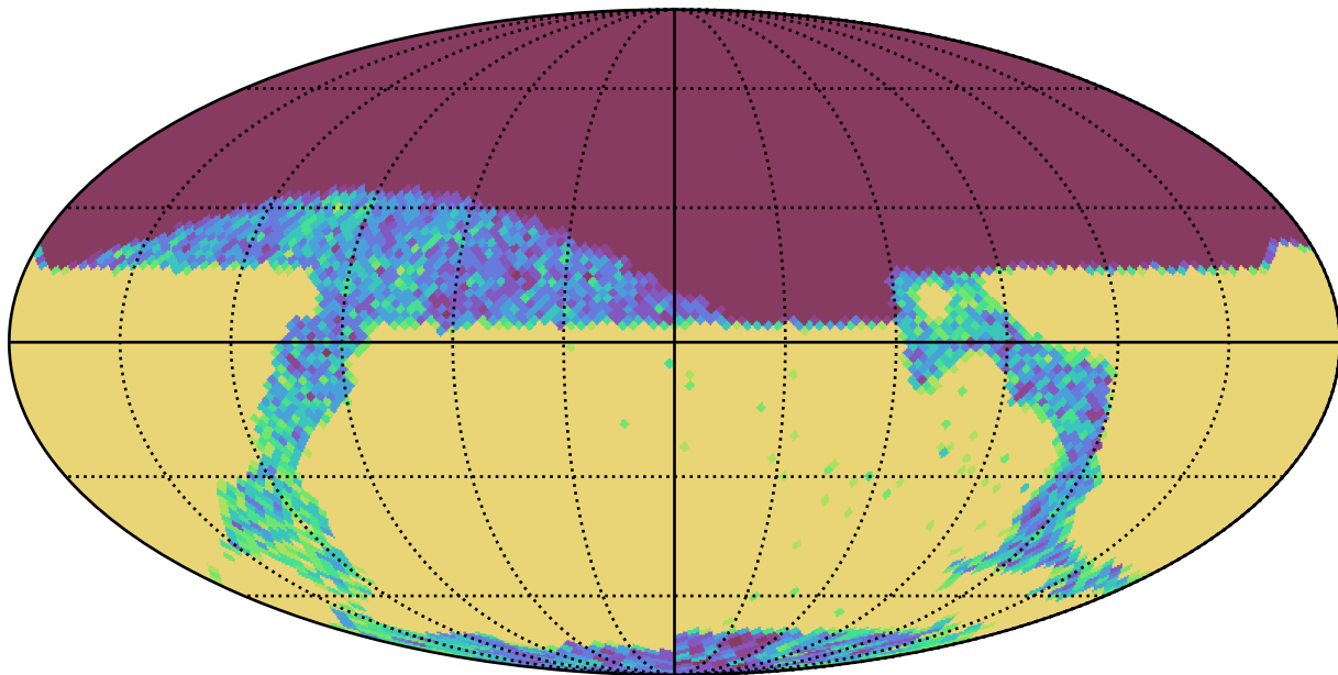
baseline_v3.0_10yrs z and night < 365: N year 1
