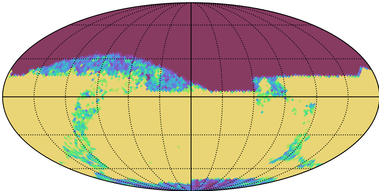
baseline_v3.0_10yrs r and night < 365: N year 1
