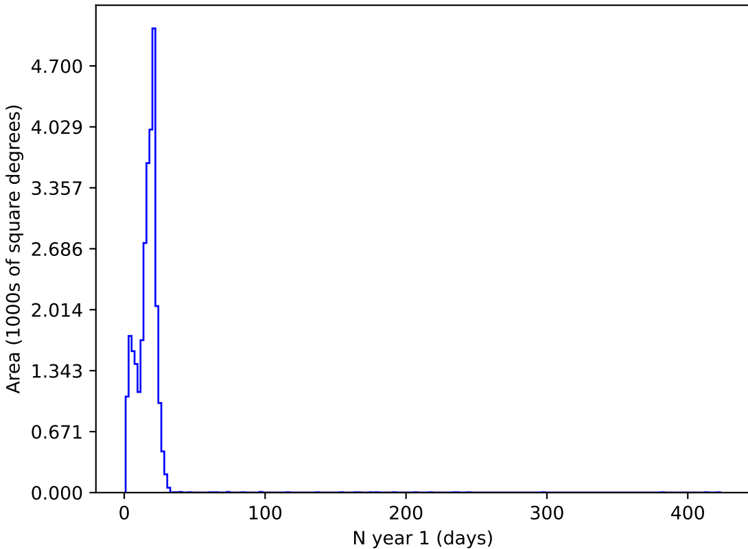
baseline_v3.0_10yrs r and night < 365: N year 1
