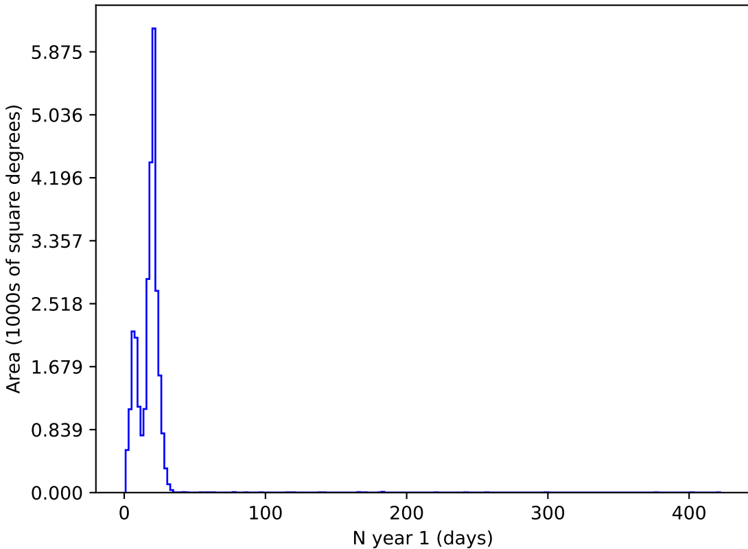
baseline_v3.0_10yrs i and night < 365: N year 1
