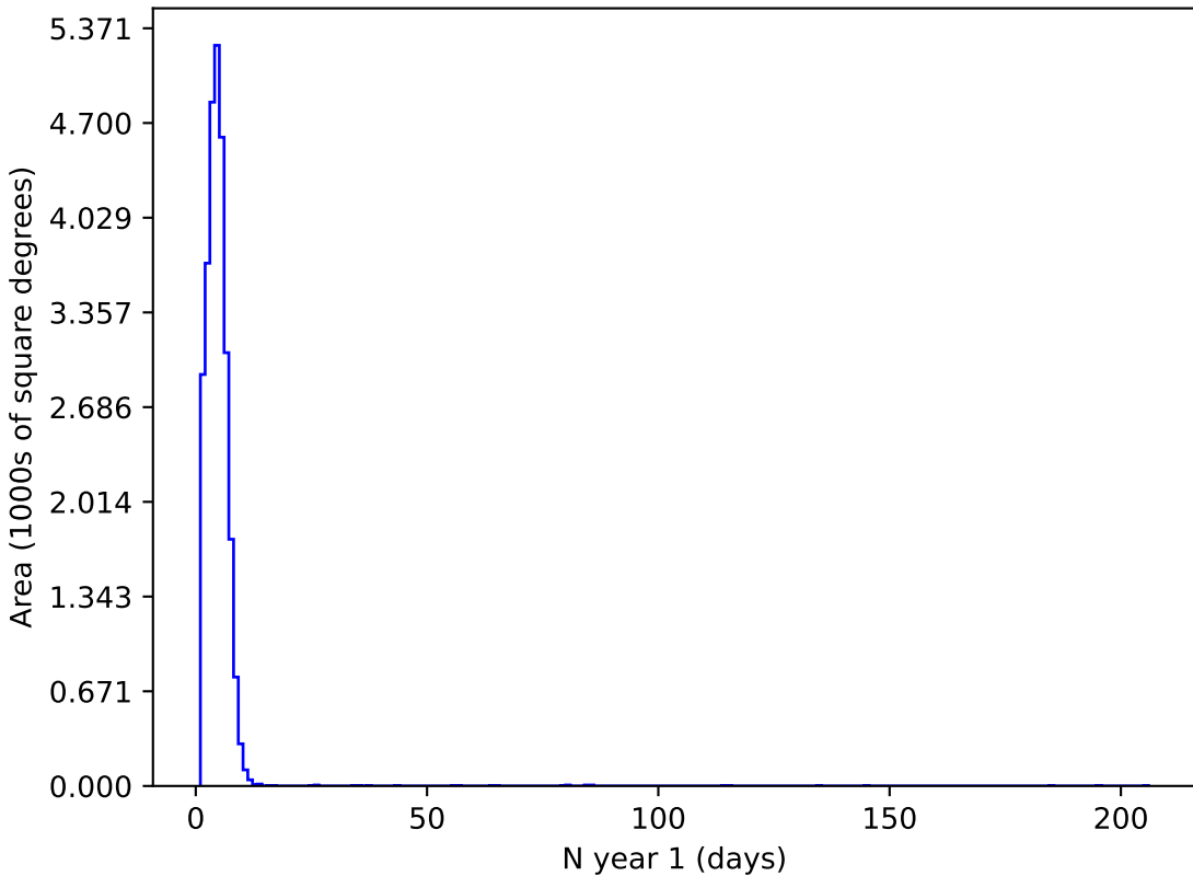
baseline_v3.0_10yrs g and night < 365: N year 1
