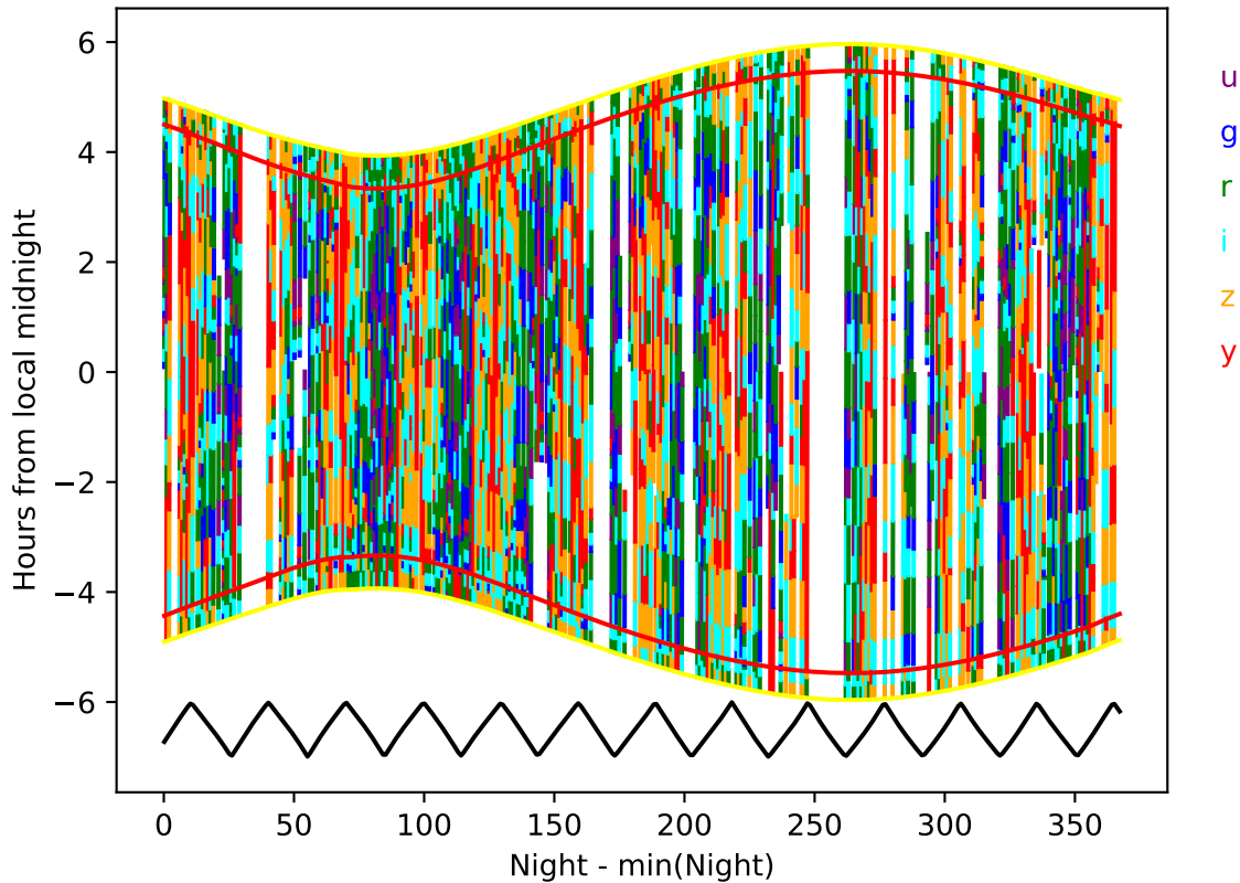
baseline_v3.0_10yrs year 7-8: Hourglass
