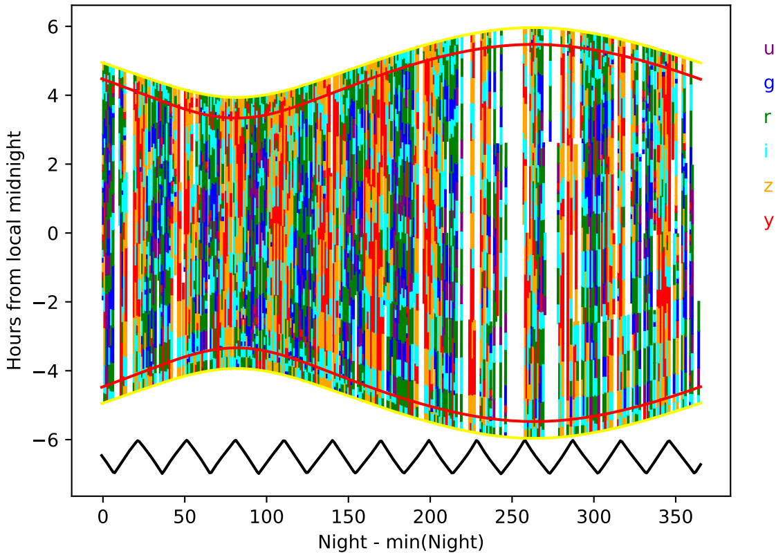
baseline_v3.0_10yrs year 6-7: Hourglass
