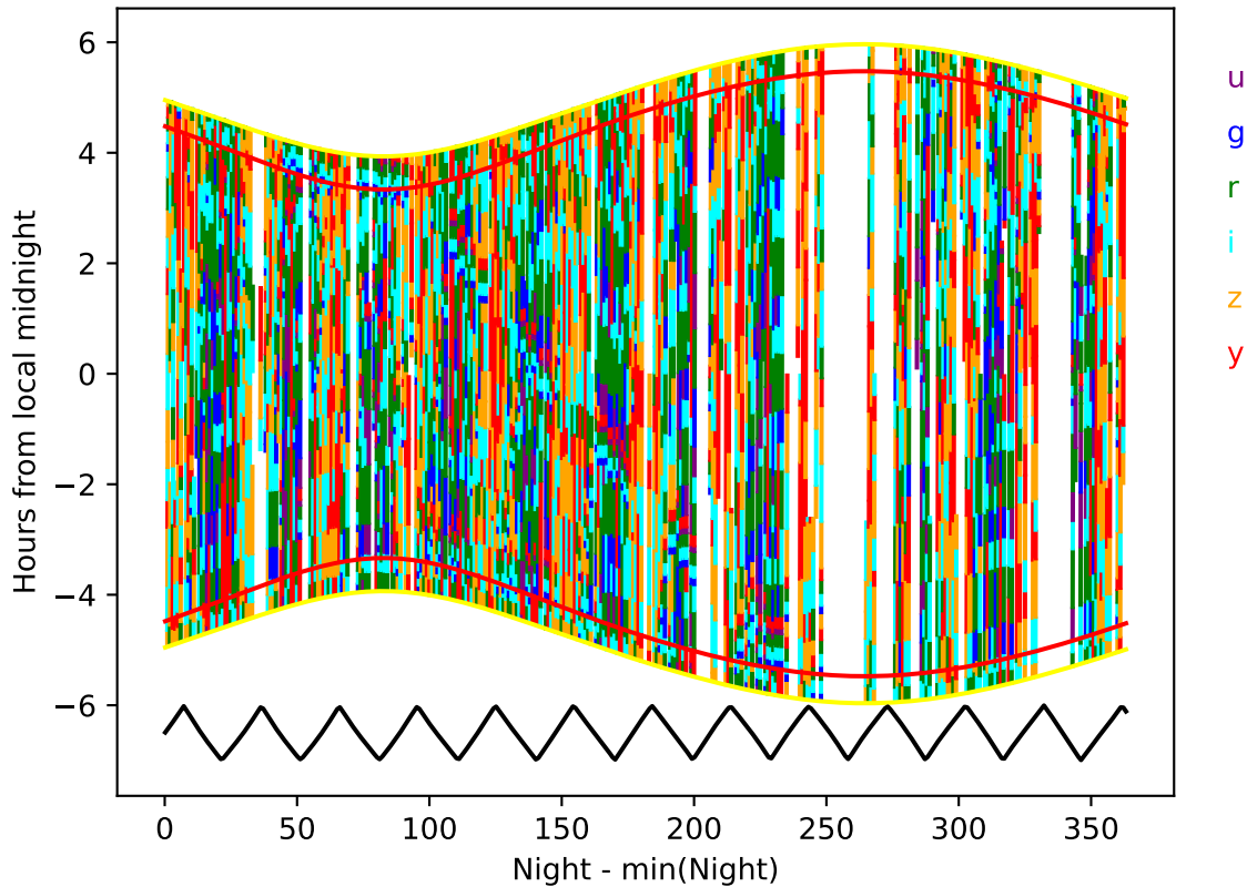
baseline_v3.0_10yrs year 2-3: Hourglass
