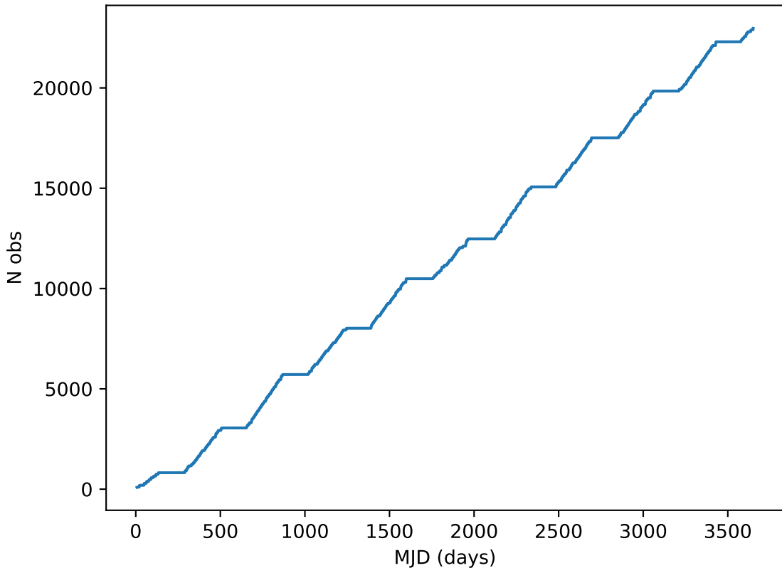
baseline_v3.0_10yrs note like DD:XMM_LSS%: Cumulative
