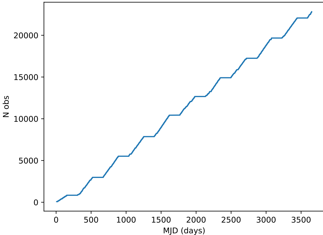
baseline_v3.0_10yrs note like DD:ECDFS%: Cumulative
