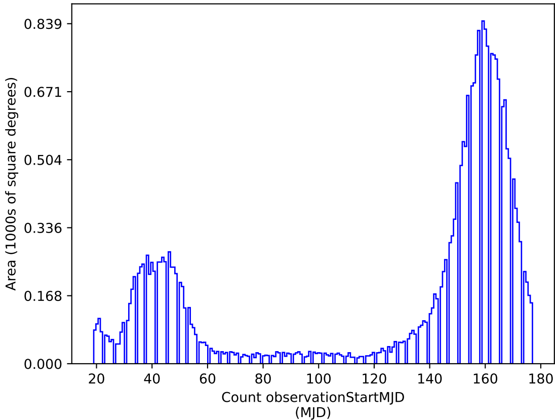
baseline_v3.0_10yrs z: Count observationStartMJD
