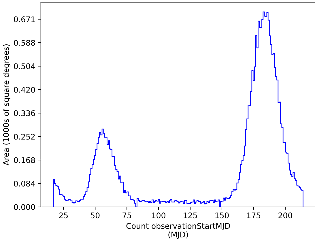
baseline_v3.0_10yrs r: Count observationStartMJD
