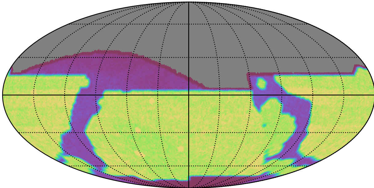
baseline_v3.0_10yrs : Count observationStartMJD
