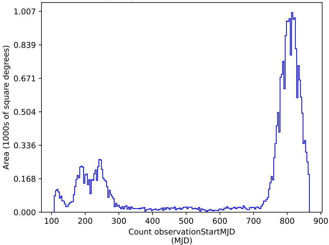
baseline_v3.0_10yrs : Count observationStartMJD
