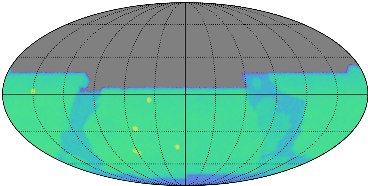
baseline_v3.0_10yrs y: CoaddM5
