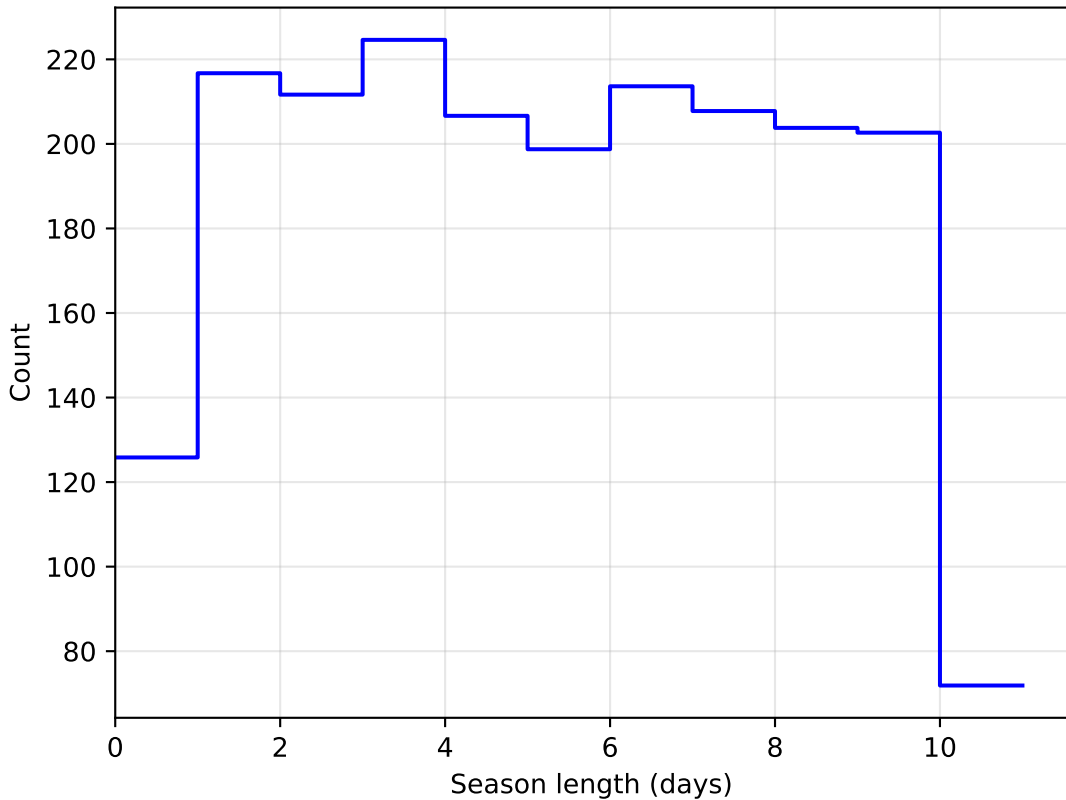
baseline_v3.0_10yrs DD:XMM_LSS all bands: SeasonLength
