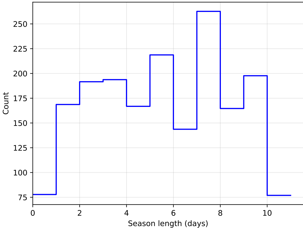
baseline_v3.0_10yrs DD:WFD all bands: SeasonLength
