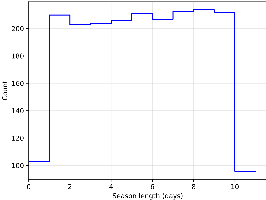
baseline_v3.0_10yrs DD:ELAISS1 all bands: SeasonLength
