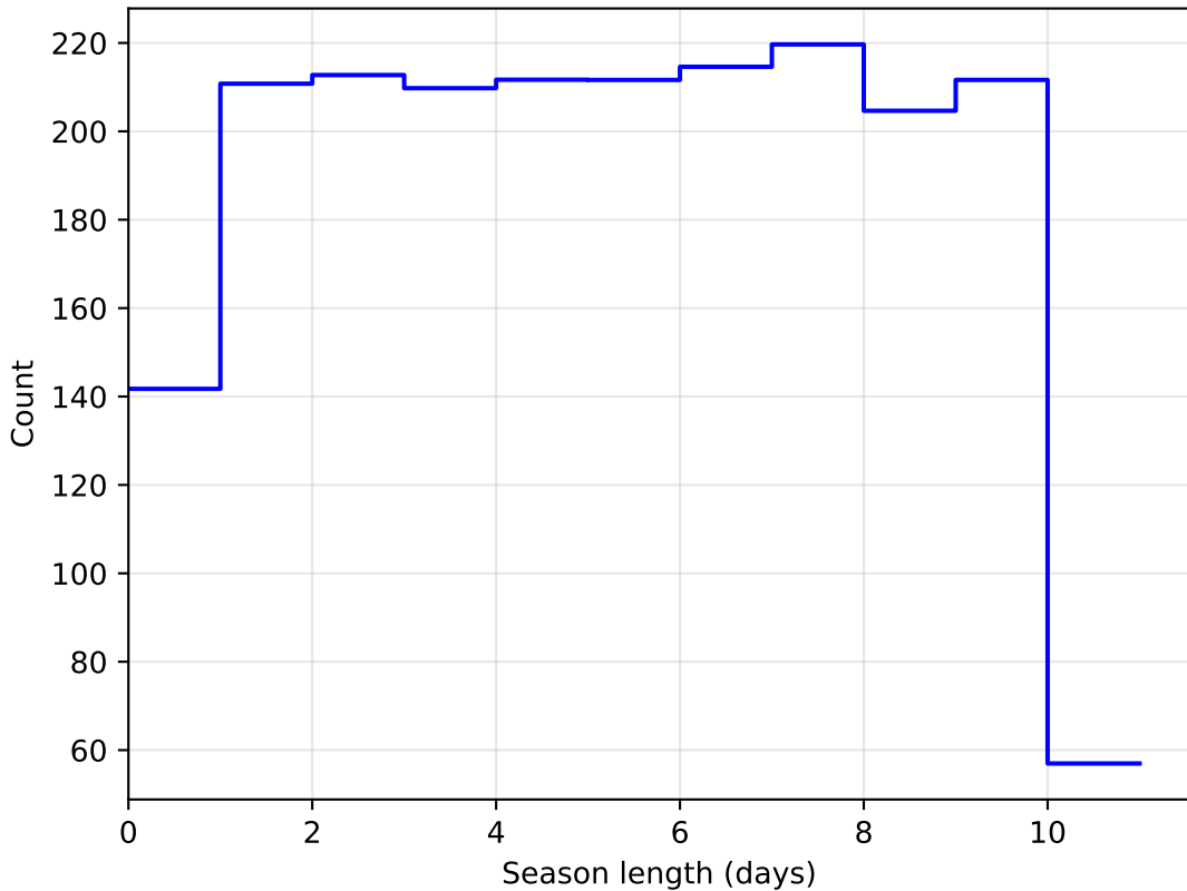
baseline_v3.0_10yrs DD:ECDFS all bands: SeasonLength
