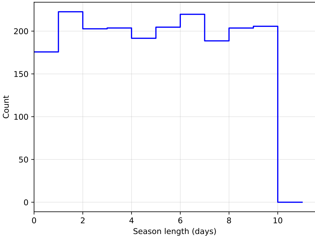
baseline_v3.0_10yrs DD: COSMOS all bands: SeasonLength
