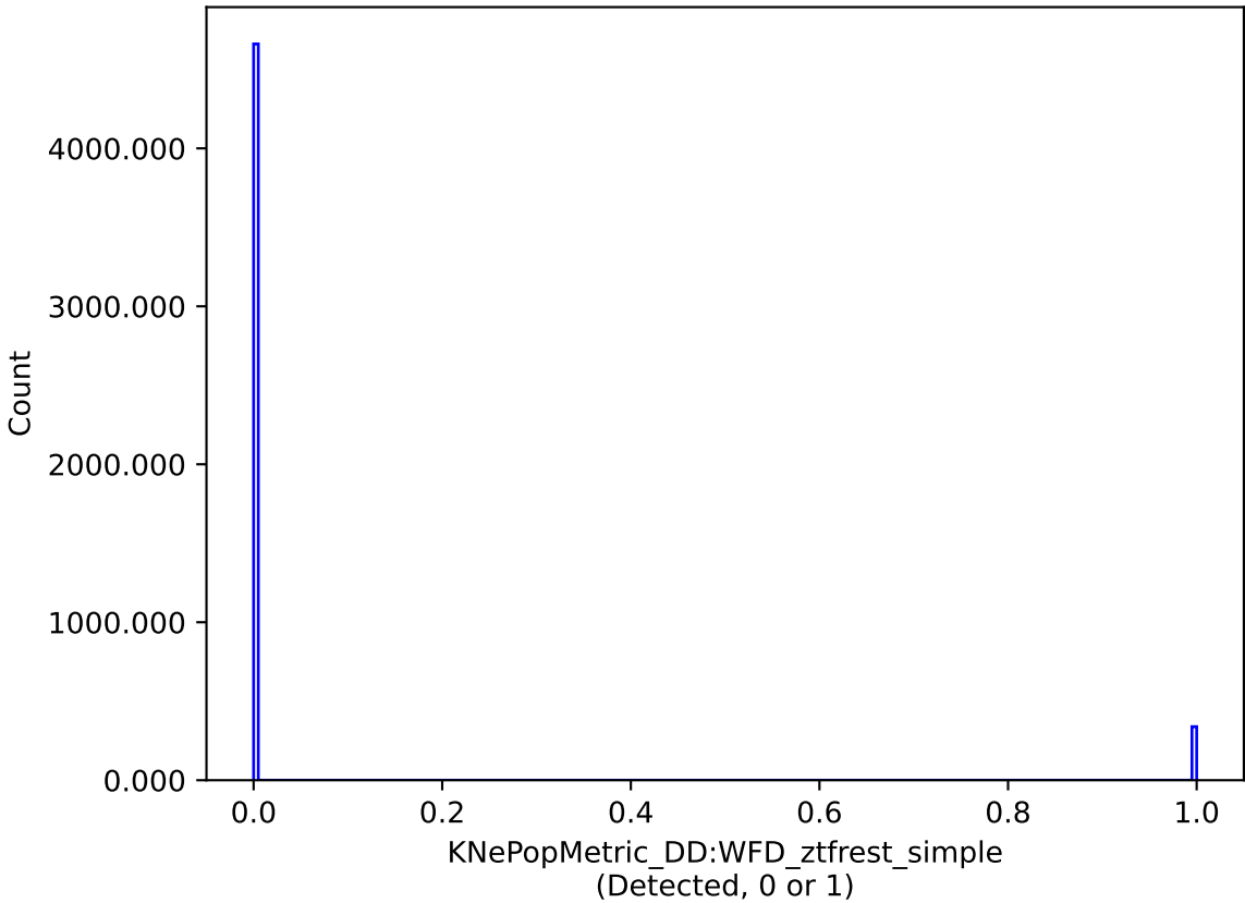
baseline_v3.0_10yrs DD:WFD: KNePopMetric_DD:WFD_ztfrest_simple
