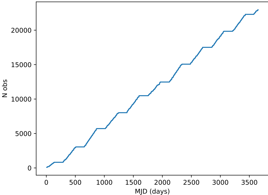
baseline_v3.0_10yrs all bands: DD:XMM_LSS Cumulative NVisits
