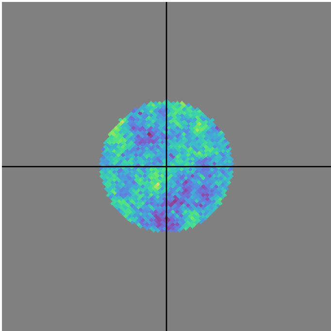
baseline_v3.0_10yrs r band: DD:WFD NVisits
