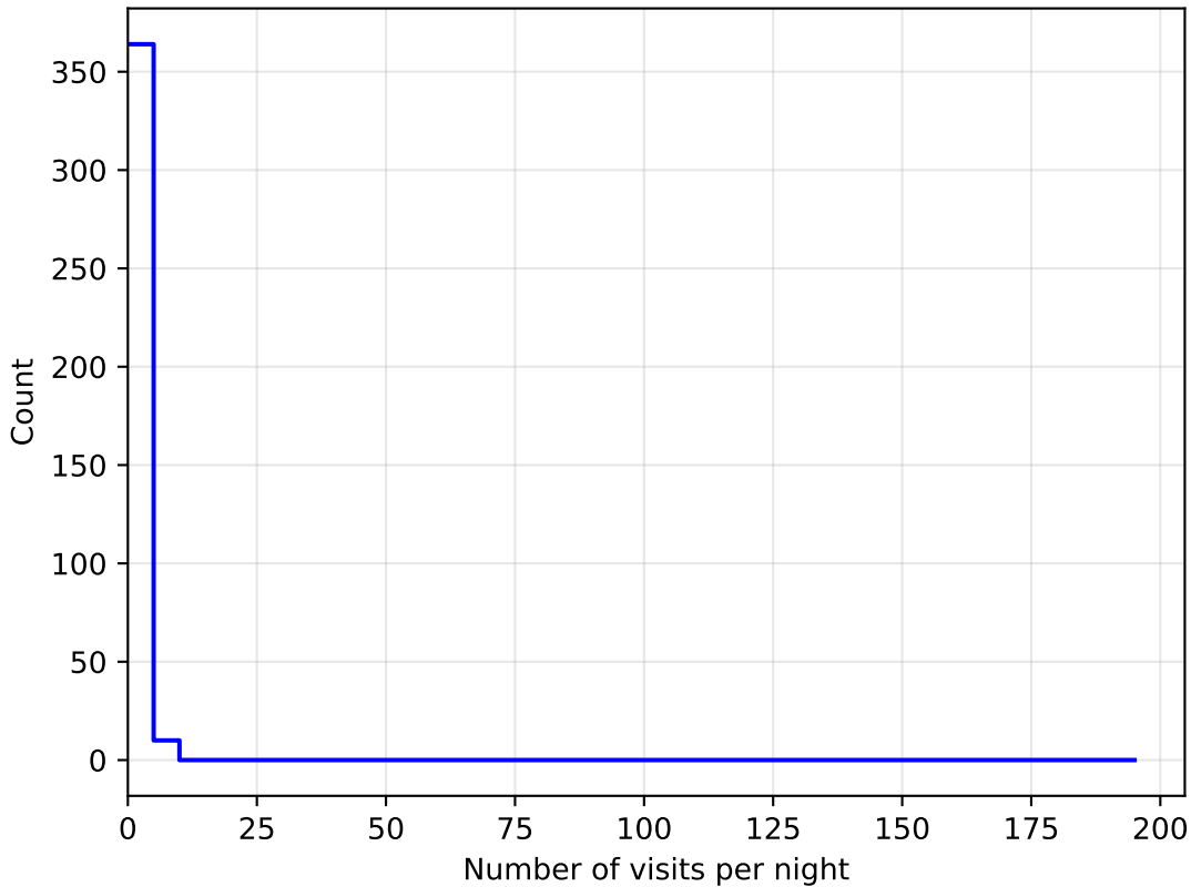
baseline_v3.0_10yrs all bands: DD:WFD NVisitsPerNight
