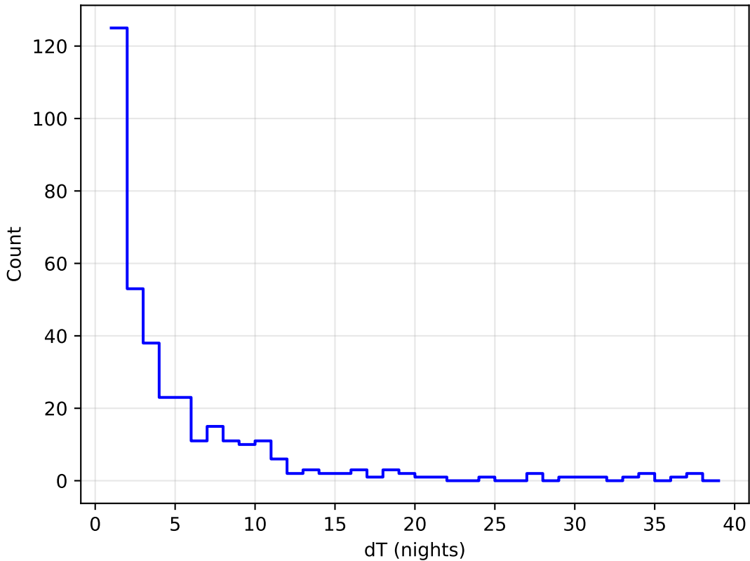
baseline_v3.0_10yrs all bands: DD:WFD Delta Nights Histogram
