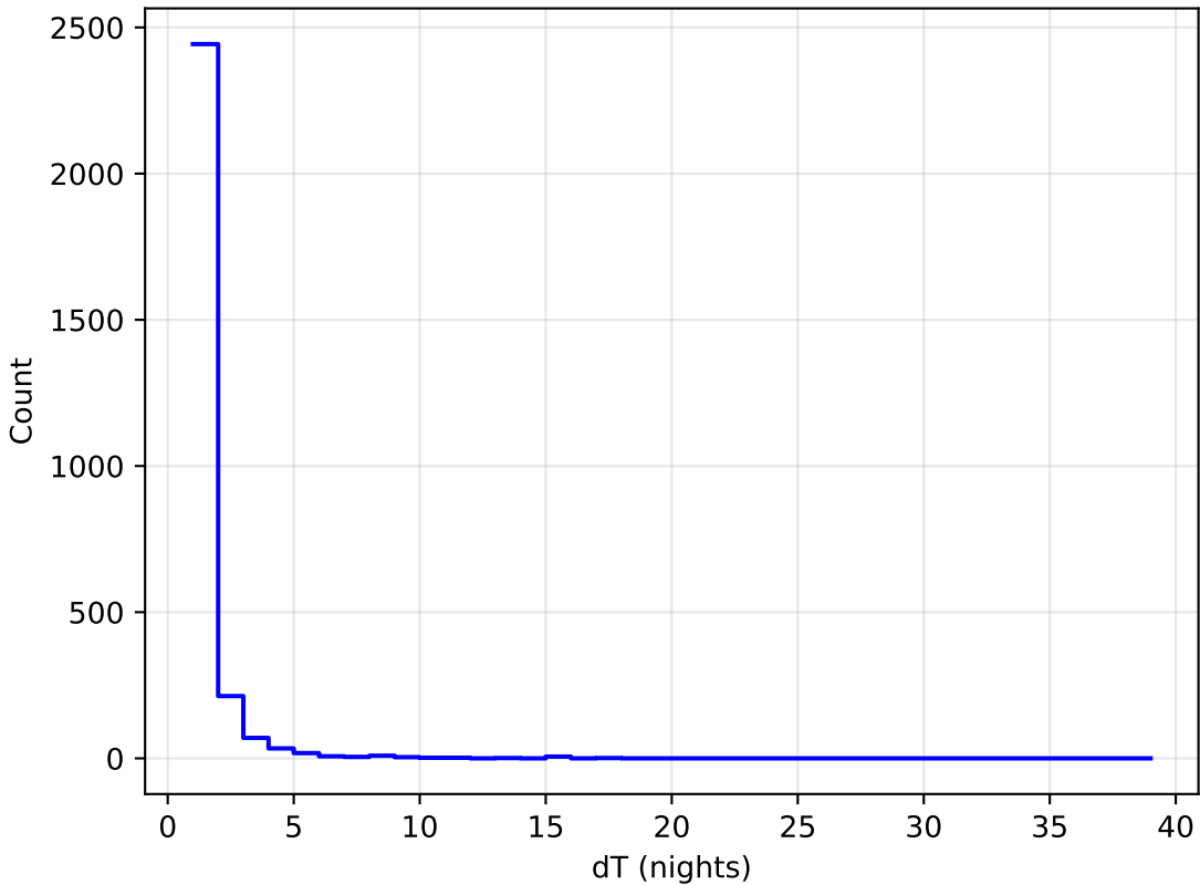
baseline_v3.0_10yrs all bands: DD:WFD Delta Nights Histogram
