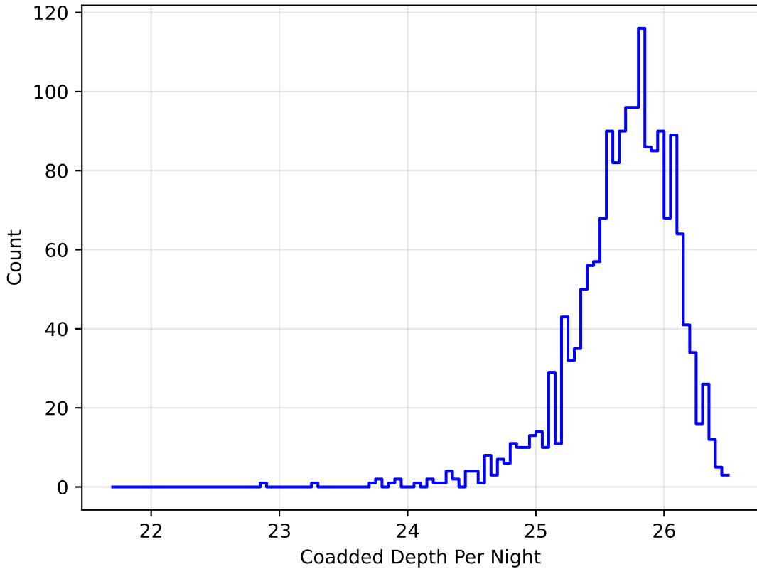
baseline_v3.0_10yrs z band: DD:WFD CoaddM5PerNight
