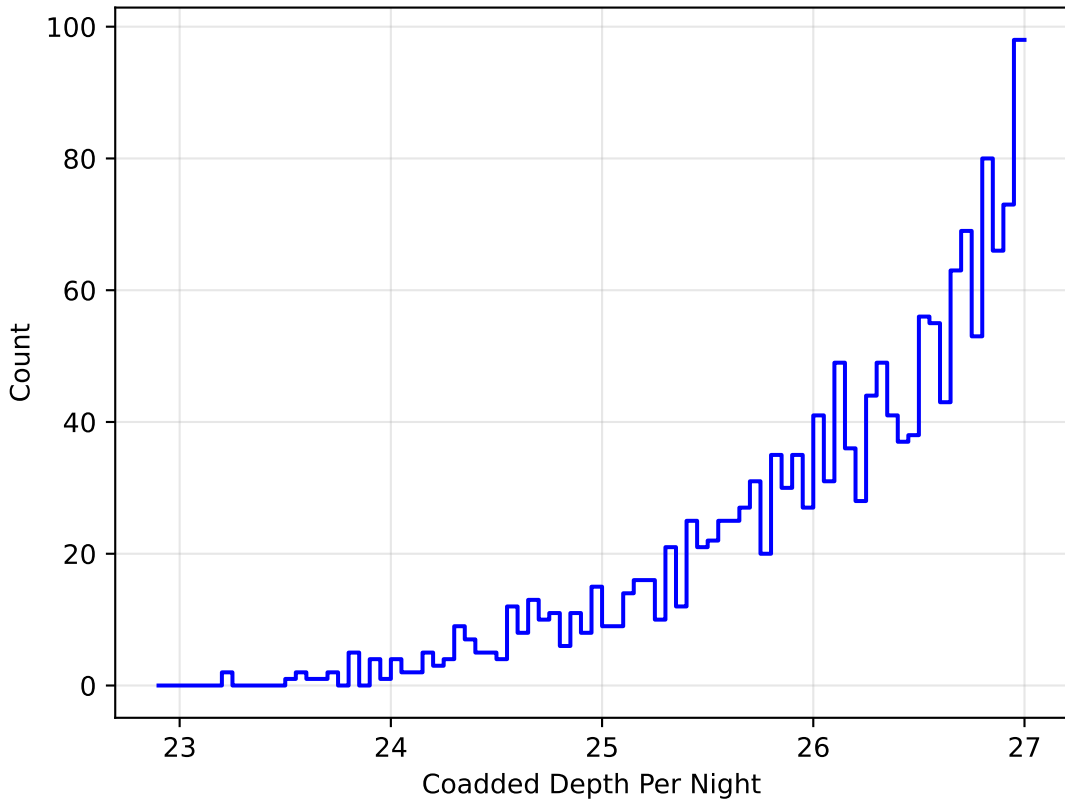
baseline_v3.0_10yrs r band: DD:WFD CoaddM5PerNight
