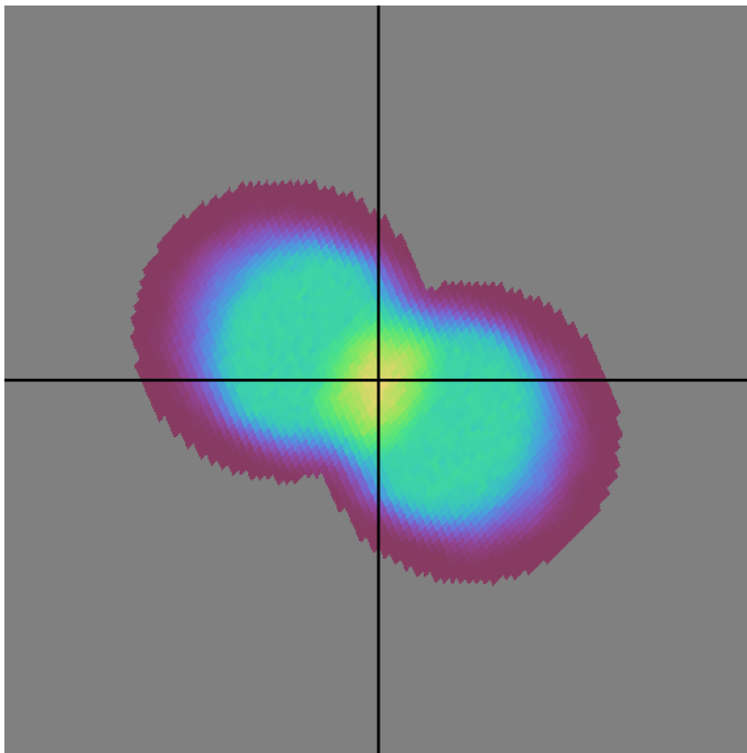
baseline_v3.0_10yrs all bands: DD:EDFS NVisits
