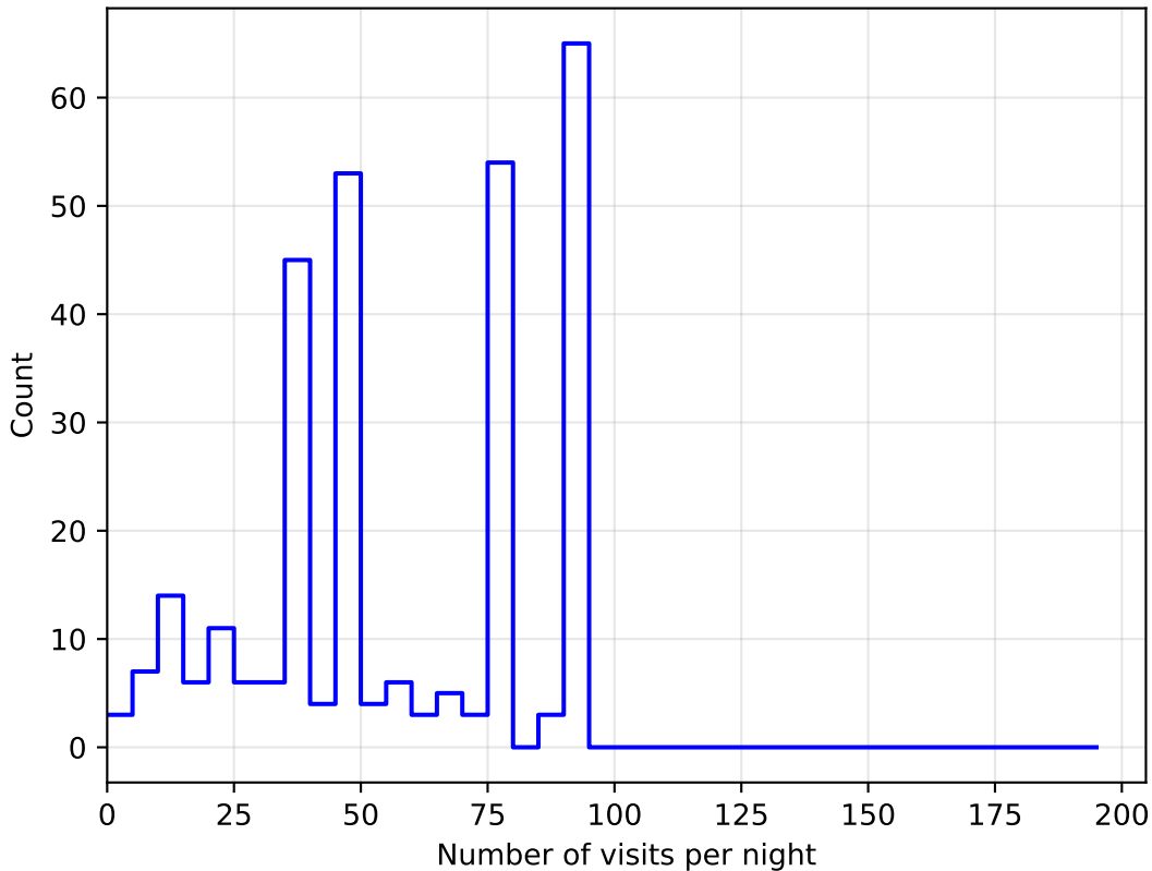
baseline_v3.0_10yrs all bands: DD:EDFS NVisitsPerNight
