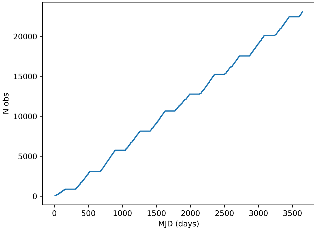
baseline_v3.0_10yrs all bands: DD:EDFS Cumulative NVisits
