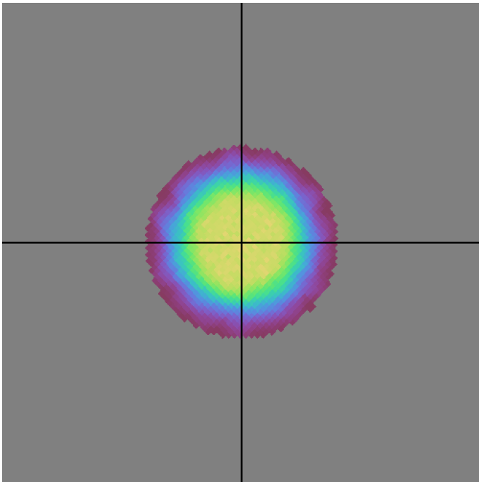
baseline_v3.0_10yrs all bands: DD:ECDFS NVisits
