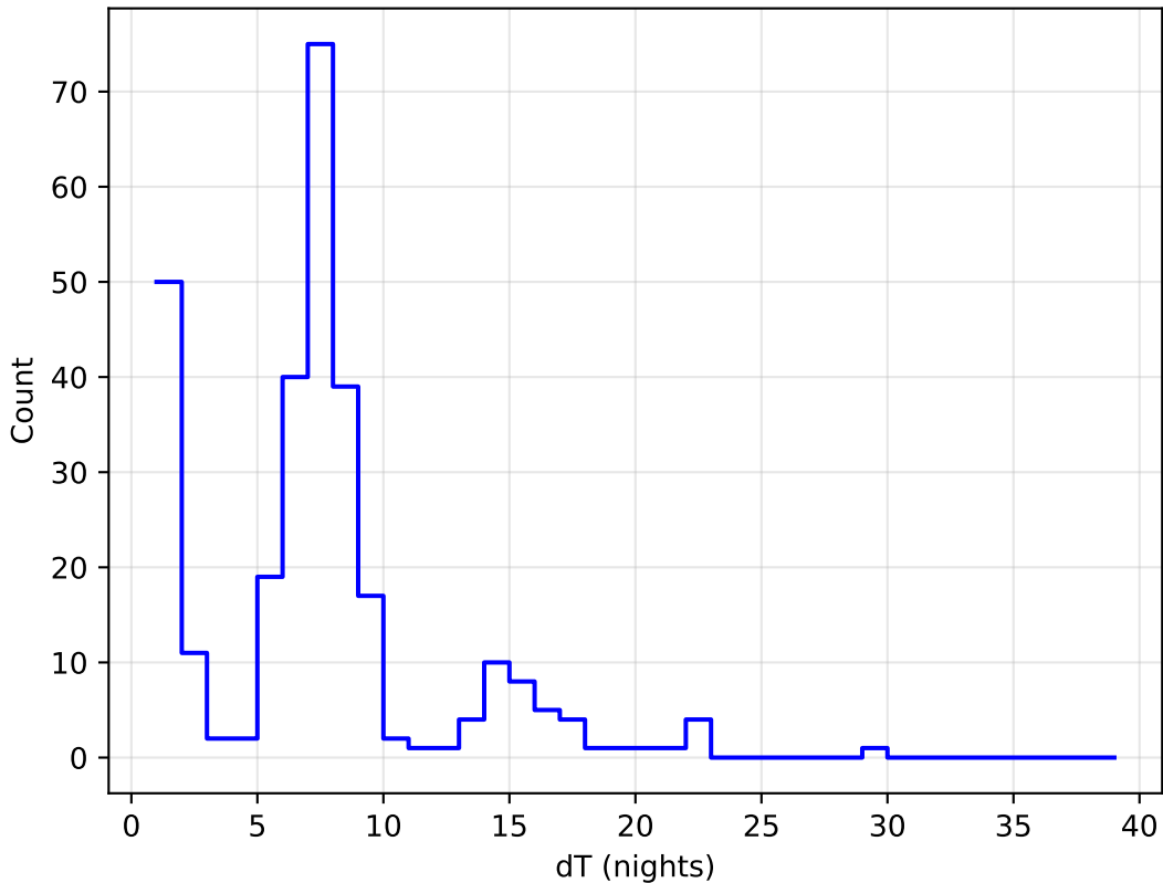
baseline_v3.0_10yrs all bands: DD:ECDFS Delta Nights Histogram
