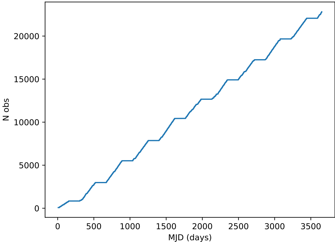
baseline_v3.0_10yrs all bands: DD:ECDFS Cumulative NVisits
