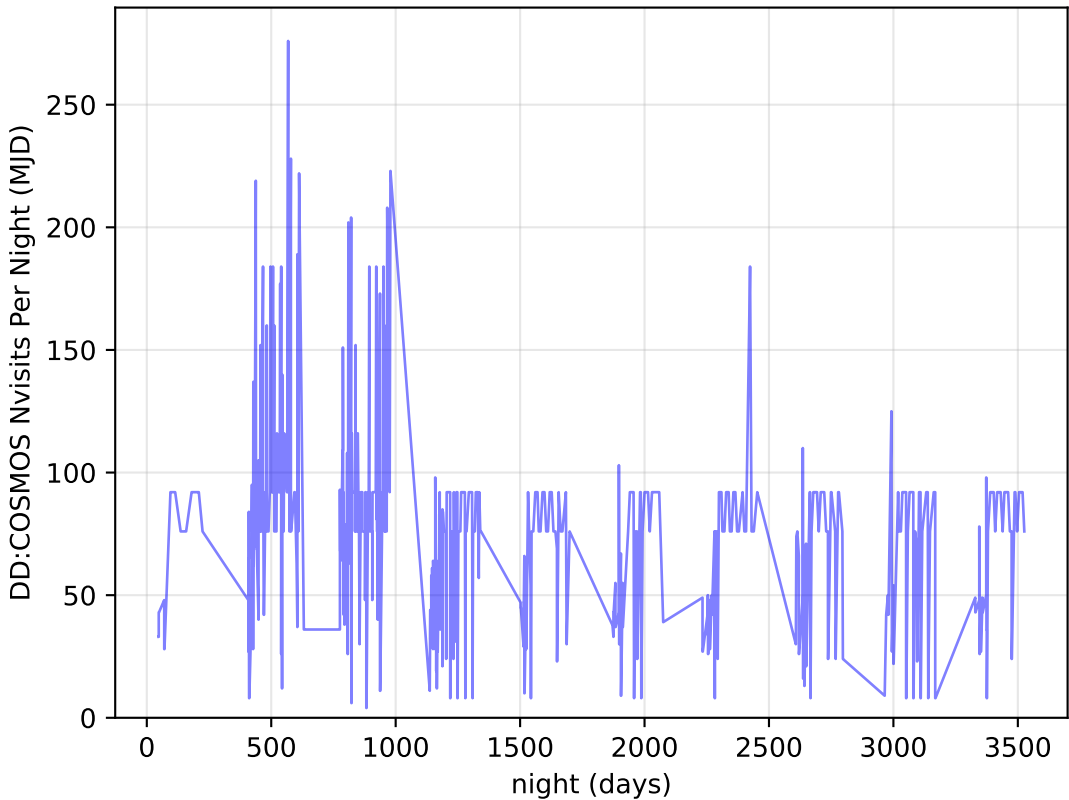
baseline_v3.0_10yrs all bands: DD:COSMOS Nvisits Per Night
