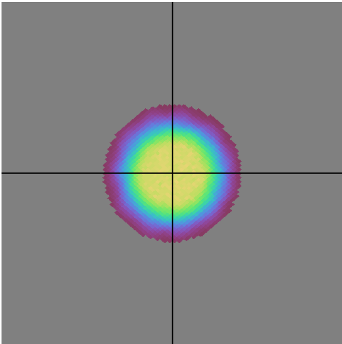
baseline_v3.0_10yrs r band: DD: COSMOS NVisits
