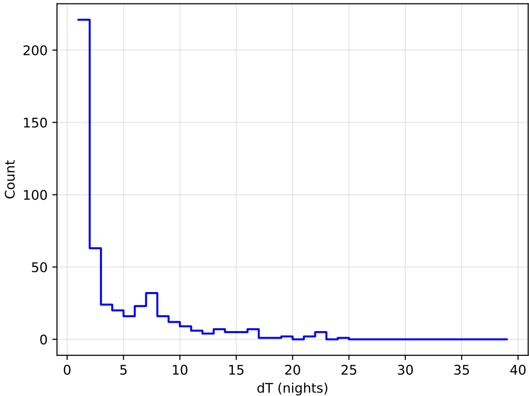
baseline_v3.0_10yrs all bands: DD: COSMOS Delta Nights Histogram
