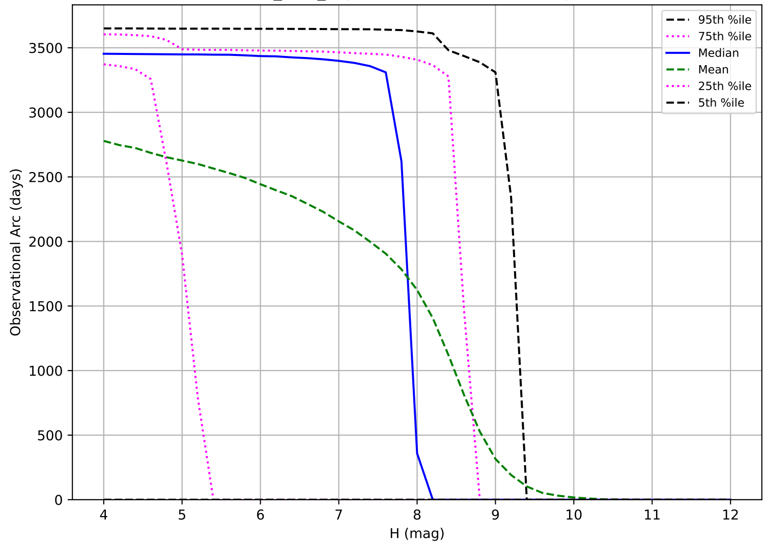
baseline_v2.1_10yrs: Observational Arc Length TNO
