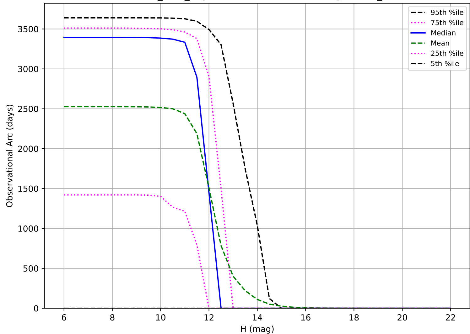
baseline_v2.1_10yrs: Observational Arc Length OCC_r20
