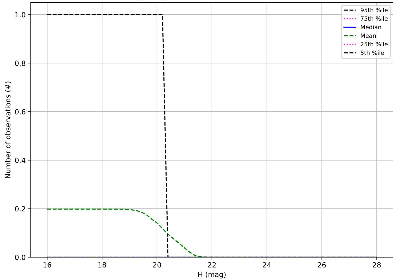
baseline_v2.1_10yrs: Number of observations Vatira
