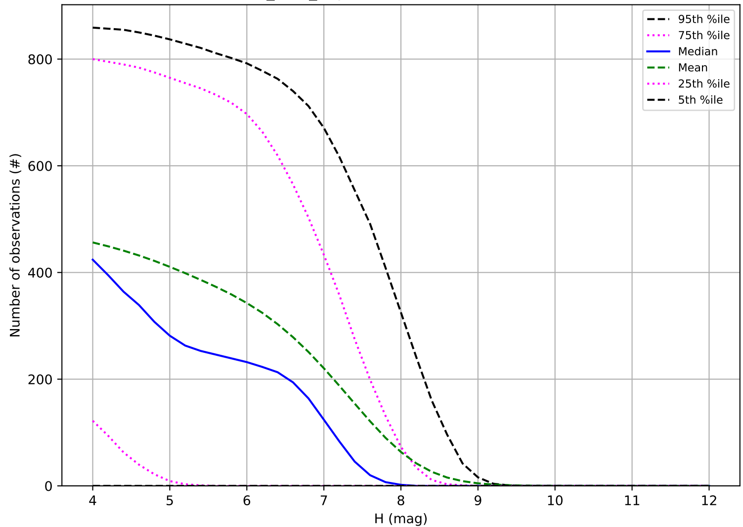
baseline_v2.1_10yrs: Number of observations TNO
