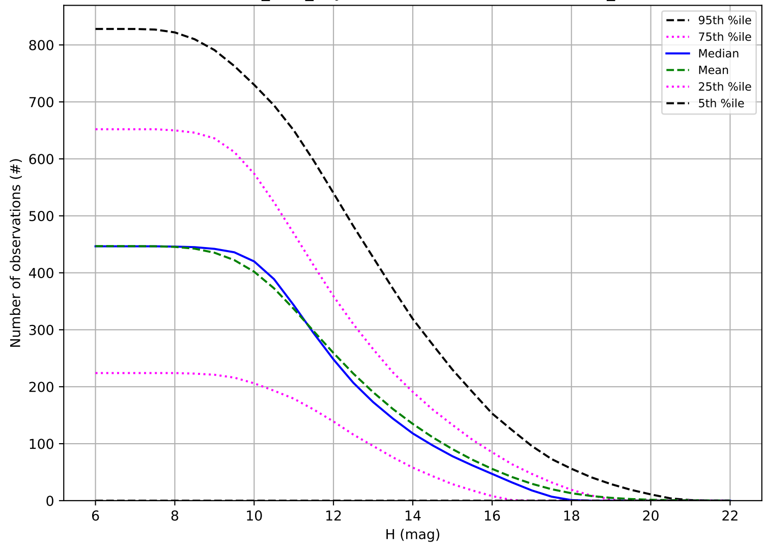
baseline_v2.1_10yrs: Number of observations OCC_r5
