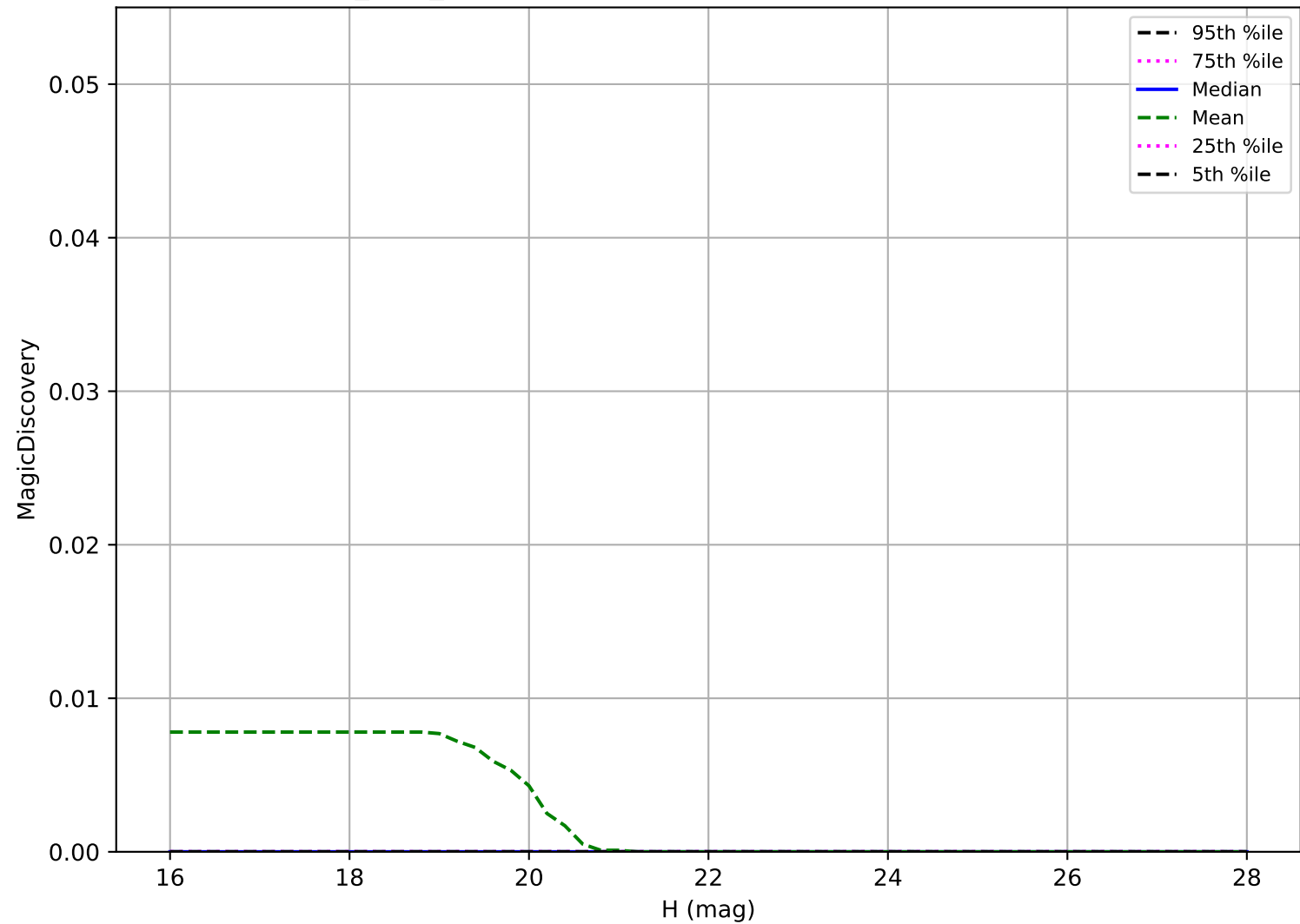
baseline_v2.1_10yrs: Vatira 6 detections in 60 nights detection loss
