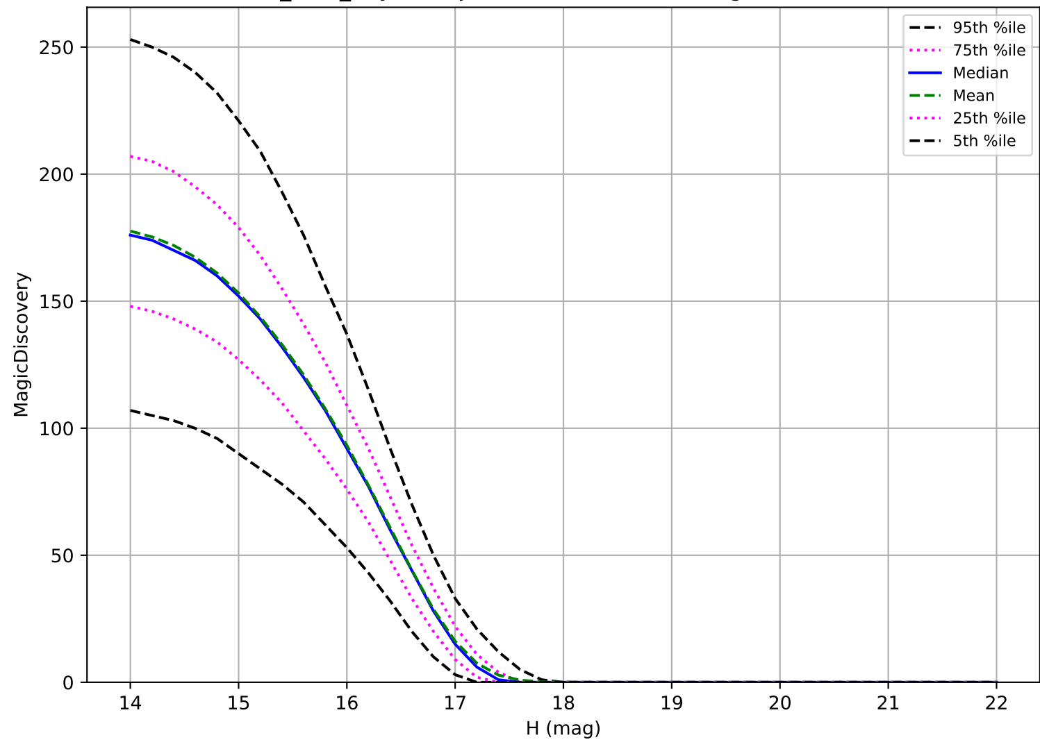
baseline_v2.1_10yrs: Trojan 6 detections in 60 nights detection loss
