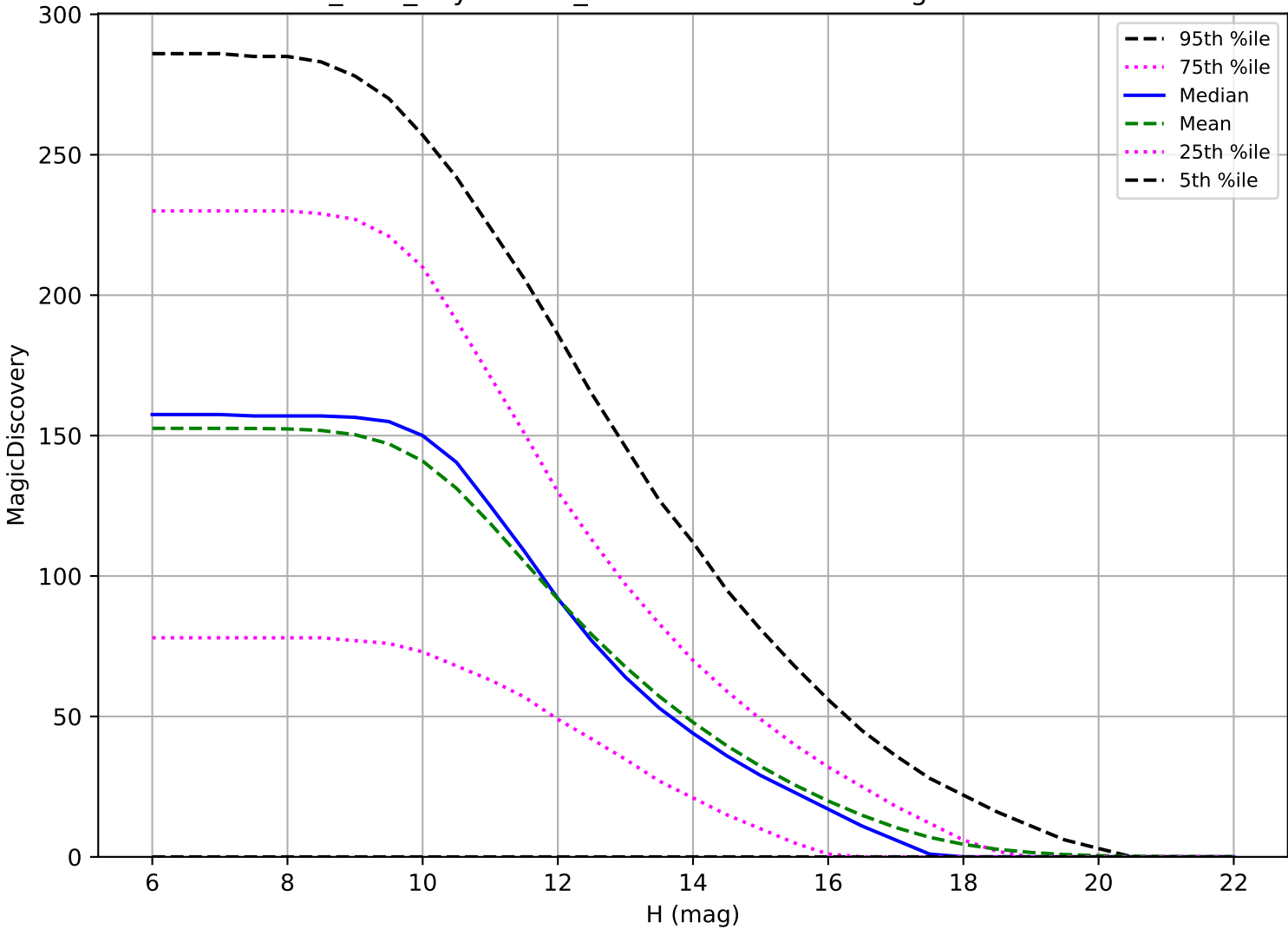
baseline_v2.1_10yrs: OCC_r5 6 detections in 60 nights detection loss
