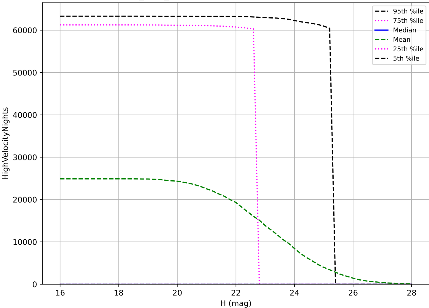
baseline_v2.1_10yrs: PHA High velocity pair detection loss
