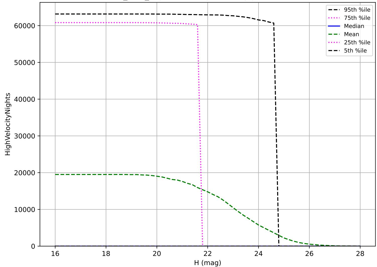
baseline_v2.1_10yrs: NEO High velocity pair detection loss
