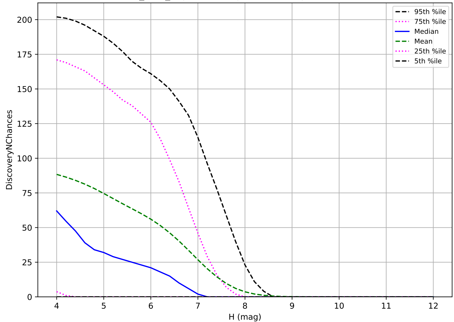
baseline_v2.1_10yrs: TNO 3 pairs in 15 nights detection loss
