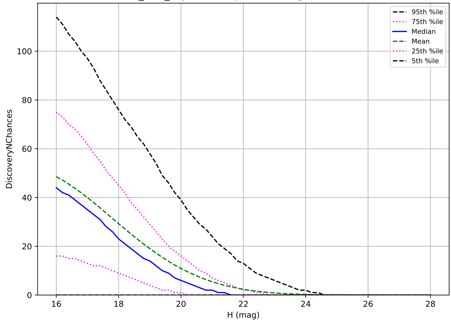
baseline_v2.1_10yrs: PHA 3 pairs in 15 nights detection loss
